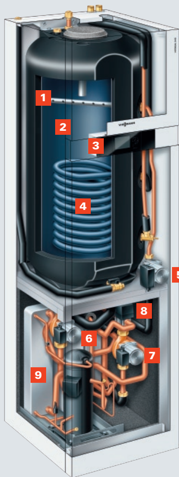
Vitocal 242-G
